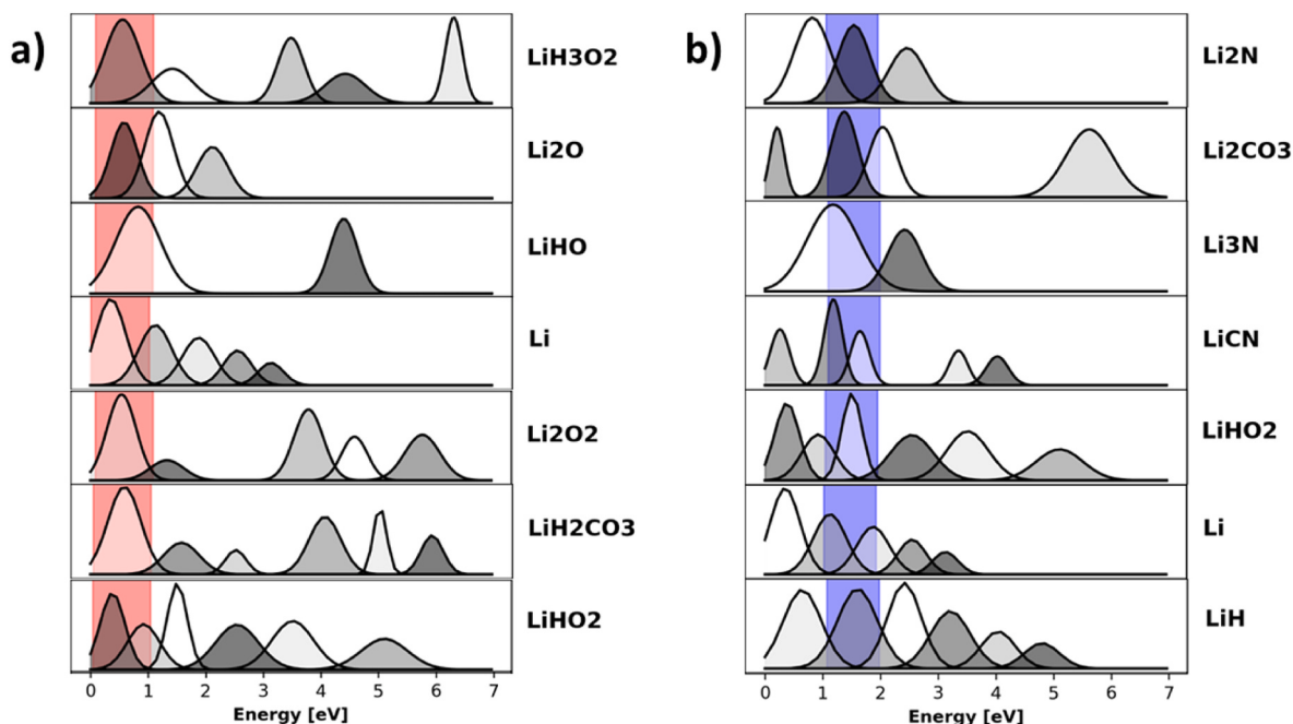
Fig. 6. (a) red (0.1–1.1 eV) and (b) blue (1.1–1.8) colour ranges overlaid onto GMMs of Li compound DOS models. The compounds are ranked by the area under the curve in each colour range. For example, the compound with the largest area under the curve in the red range was \text{LiH}_3\text{O}_2 .
