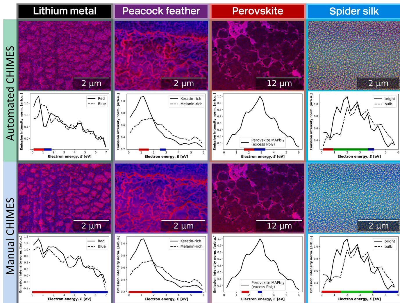
Fig. 5. Comparison of automated and manual CSEHI results, with their respective spectral colour ranges.
